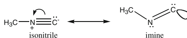
Scheme 1 Resonance structures for methyl isocyanide
