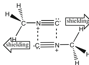
Scheme 2 Proposed methyl isocyanide dimer in nonpolar solvent
